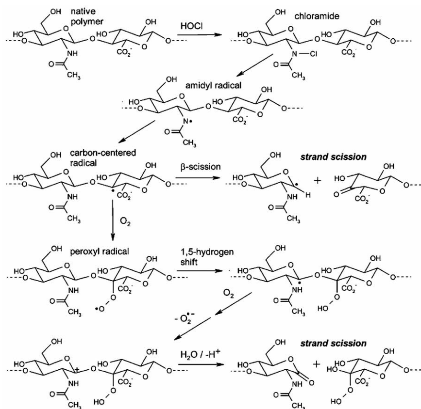
Fig. (5). Degradative pathway of HA initiated by \text{HOCl} action on the N -acetyl group. Reprinted with permission from [107].
