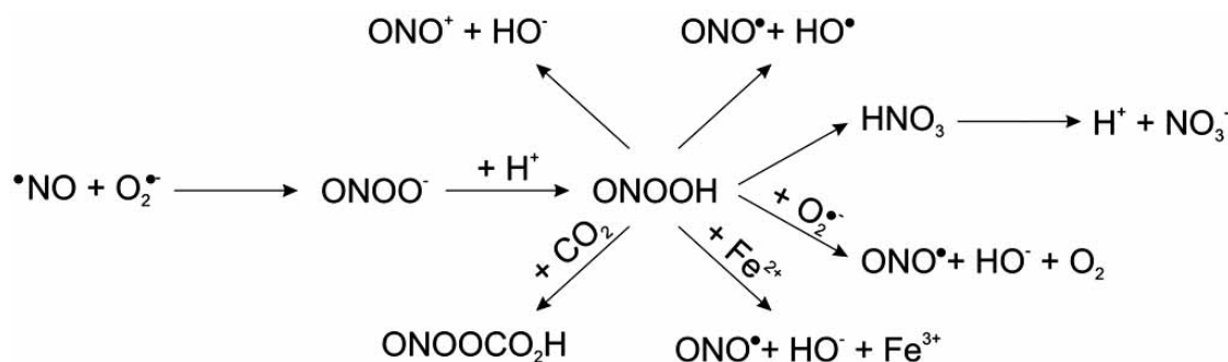
Fig. (6). In vivo generation of peroxynitrite ( \text{ONOO}^- ) as well as important decay mechanisms of this compound. For details see text.
